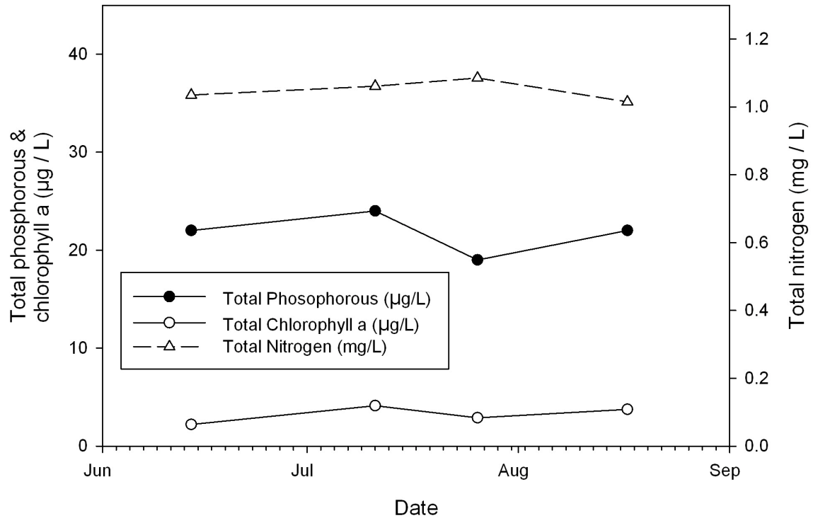
Figure 4. Total phosphorous, chlorophyll a (a measure of algal biomass), and total nitrogen concentrations for Arm Lake during the summer of 2009.
