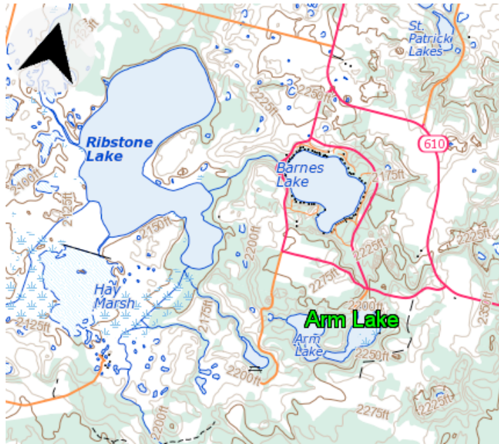
Figure 1. Topographic map of Arm Lake, Alberta and surroundings. Atlas of Canada, 2010.
