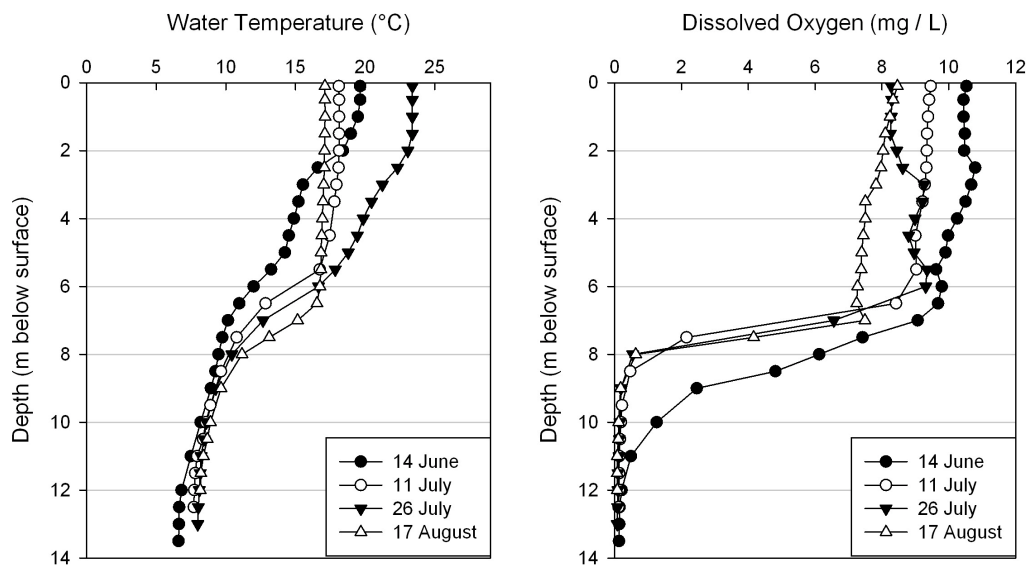
Figure 3. Water temperature (°C) and dissolved oxygen (mg/L) profiles for Arm Lake during the summer of 2009.
