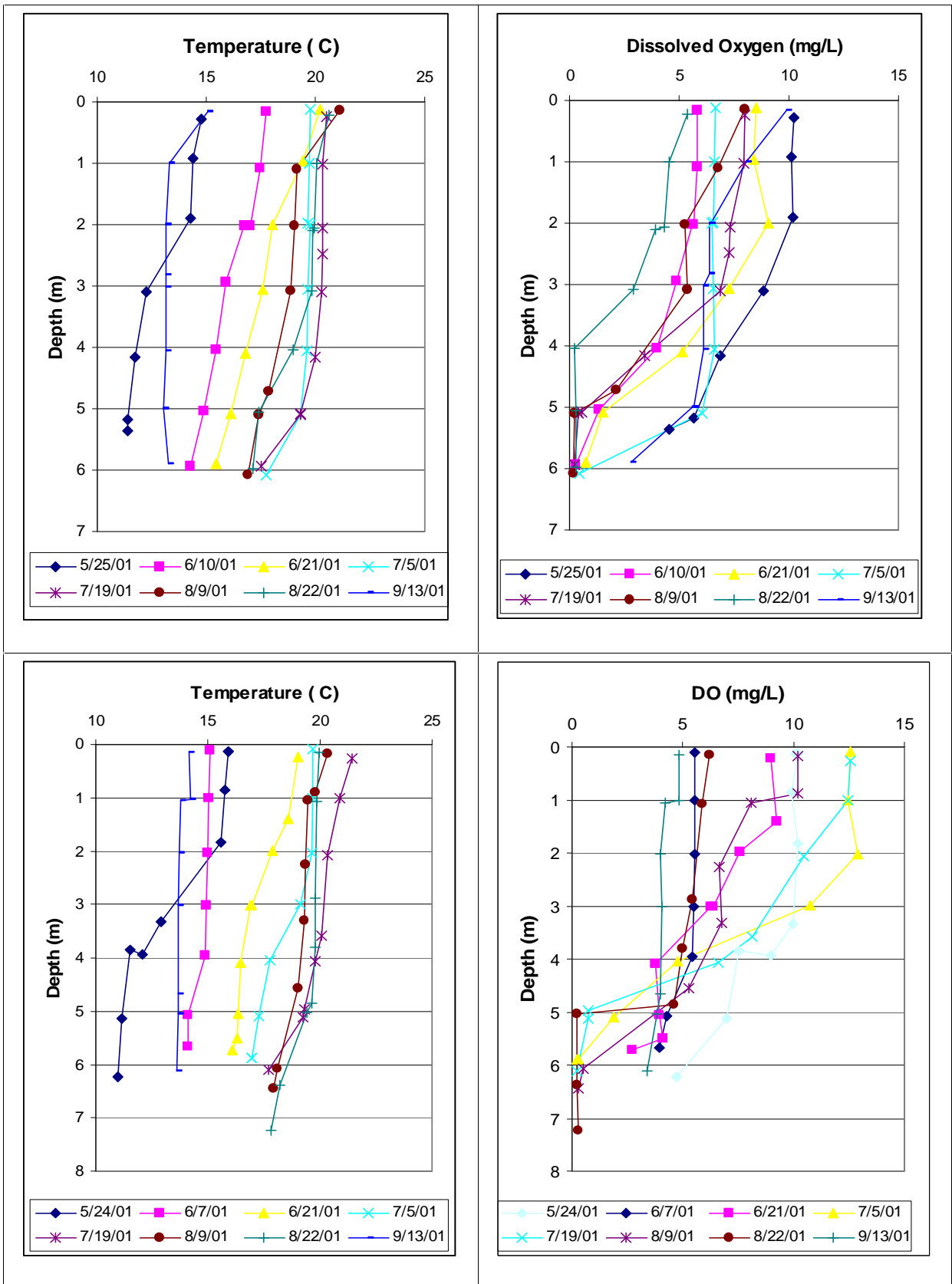
Fig. 4: Temperature and dissolved oxygen profiles for Middle and South Chain Lakes.
