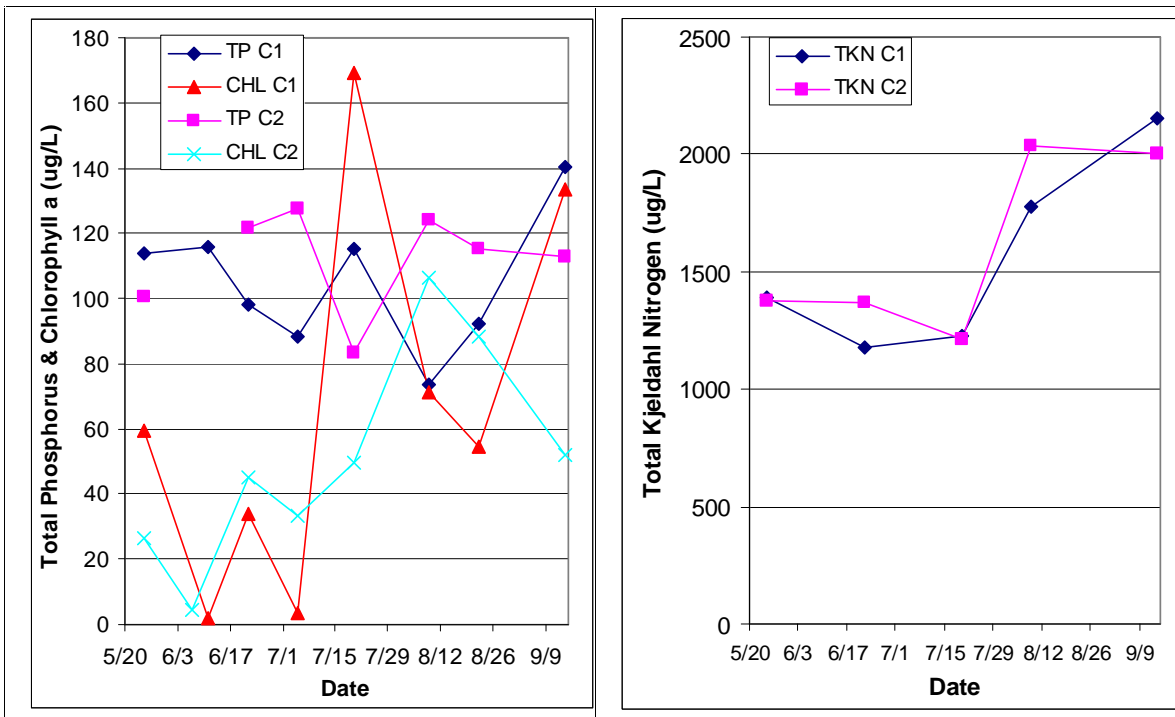
Fig. 5 & 6: Total phosphorus and chlorophyll a and total Kjeldahl nitrogen for middle (C1) and south (C2) Chain Lake during summer 2001.
