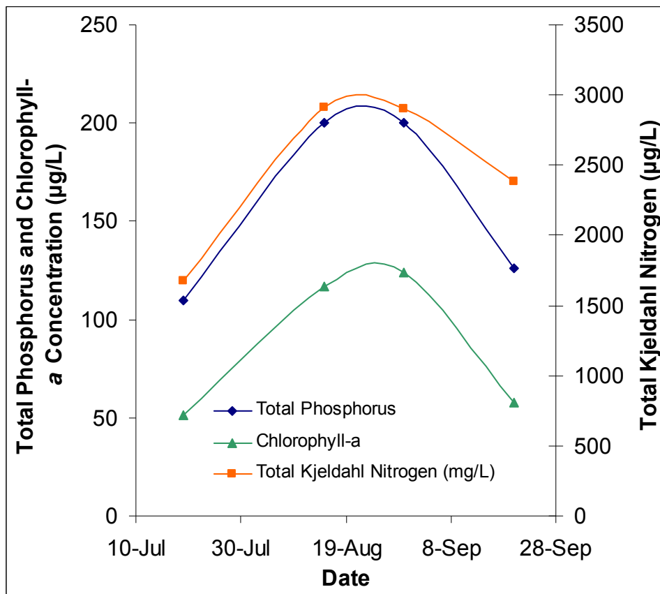
Figure 3 – Total phosphorus ( \mu\text{g}/\text{L} ), chlorophyll- a concentration ( \mu\text{g}/\text{L} ), and total Kjeldahl nitrogen ( \mu\text{g}/\text{L} ) measured four times over the course of the summer at Chip Lake.
