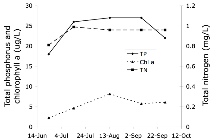
Figure 4: Total phosphorus, total nitrogen, and chlorophyll a (a measure of algae biomass or water greenness) concentrations for Clear Lake during the summer of 2006.
