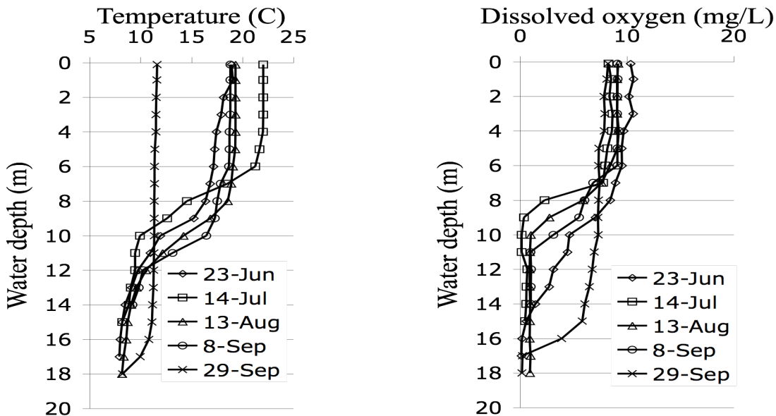
Figures 3: Water temperature and dissolved oxygen profiles for Clear Lake during the summer of 2006.
