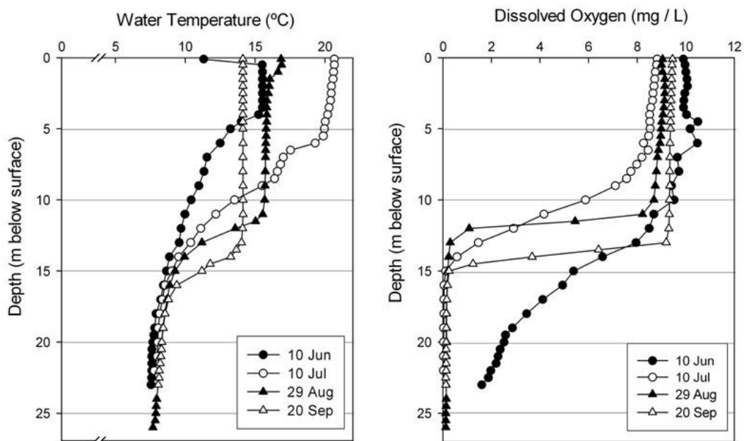
Figure 4. Water temperature ( ^{\circ}\text{C} ) and dissolved oxygen ( \text{mg / L} ) profiles for Crane (Moore) Lake during the summer of 2007.
