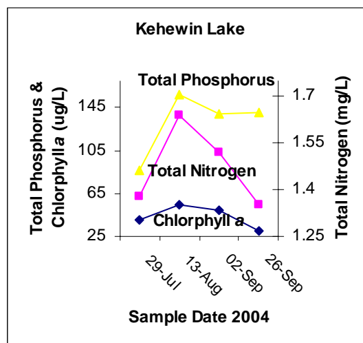
Figure 6. Total phosphorus, total nitrogen and chlorophyll a (i.e., water greenness) concentrations, summer 2004.
