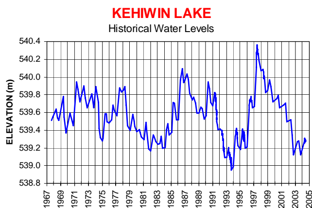
Figure 3. Historical water levels for Kehewin Lake.
