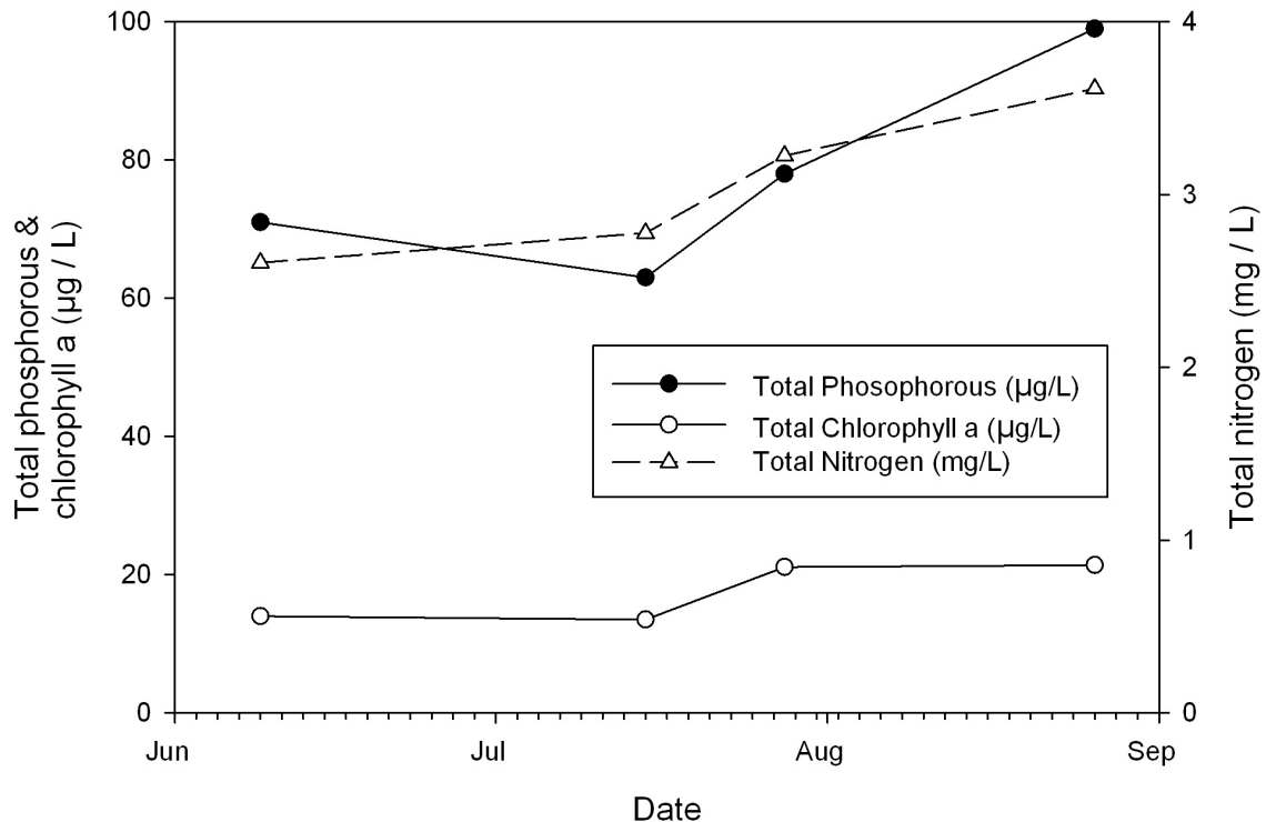
Figure 5. Total phosphorous, chlorophyll a (a measure of algal biomass), and total nitrogen concentrations for Kinosiu Lake during the summer of 2009.
