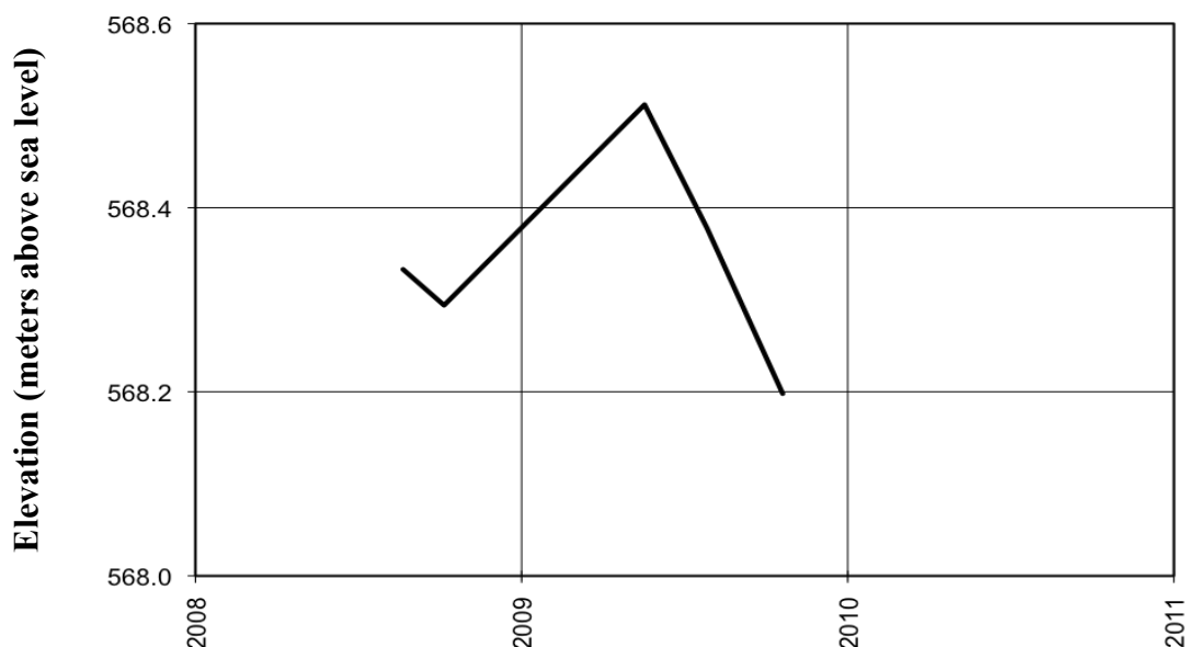
Figure 3. Historical water levels (m asl) in Kinosisu Lake, Alberta 2008 – 2009.
