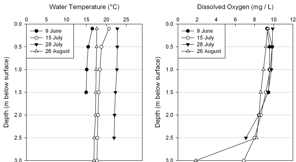
Figure 4. Water temperature (°C) and dissolved oxygen (mg/L) profiles for Kinosisu Lake during the summer of 2009.
