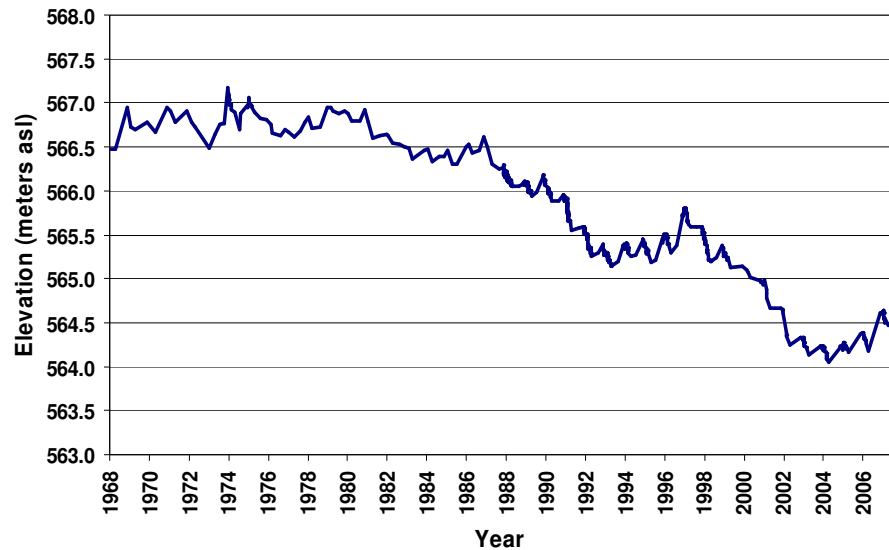
Figure 3. Historical water level elevation (meters above sea level (asl)) in Laurier Lake, Alberta, 1968-2007.
