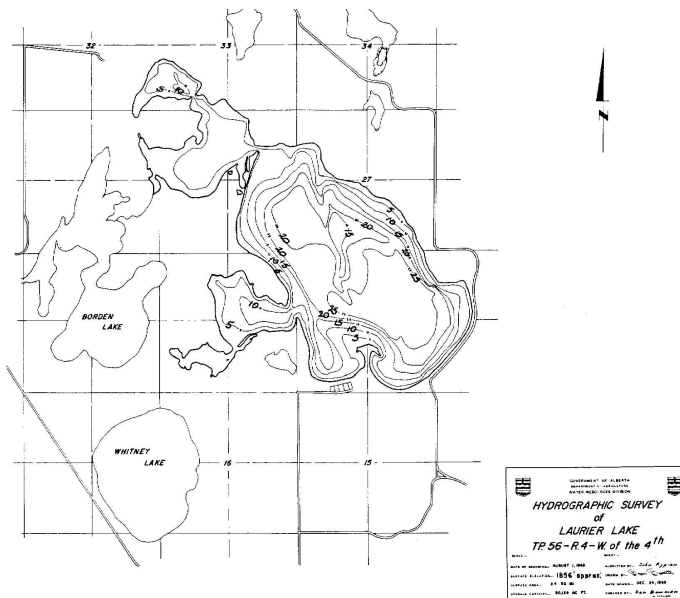
Figure 2. Bathymetry of Laurier Lake, Alberta. Contours are at 5 ft. intervals
