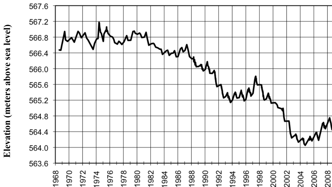
Figure 3. Historical water levels (meters above sea level (asl)) in Laurier Lake, Alberta 1968 – 2009.
