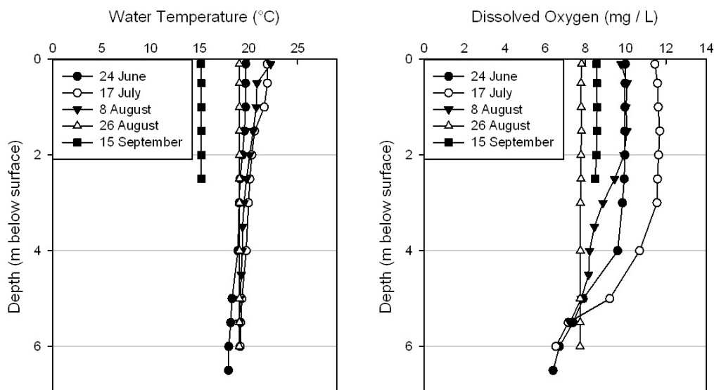
Figure 4. Water temperature (°C) and dissolved oxygen (mg/L) profiles for Laurier Lake during the summer of 2008.
