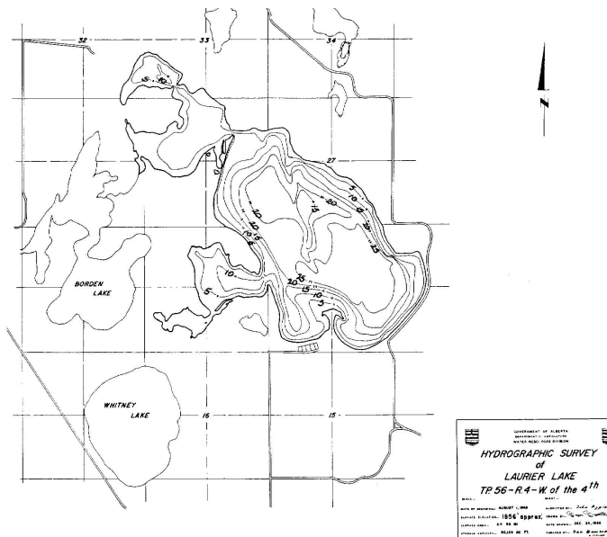
Figure 2. Bathymetry of Laurier Lake, Alberta. Contours are at 5 ft. intervals
