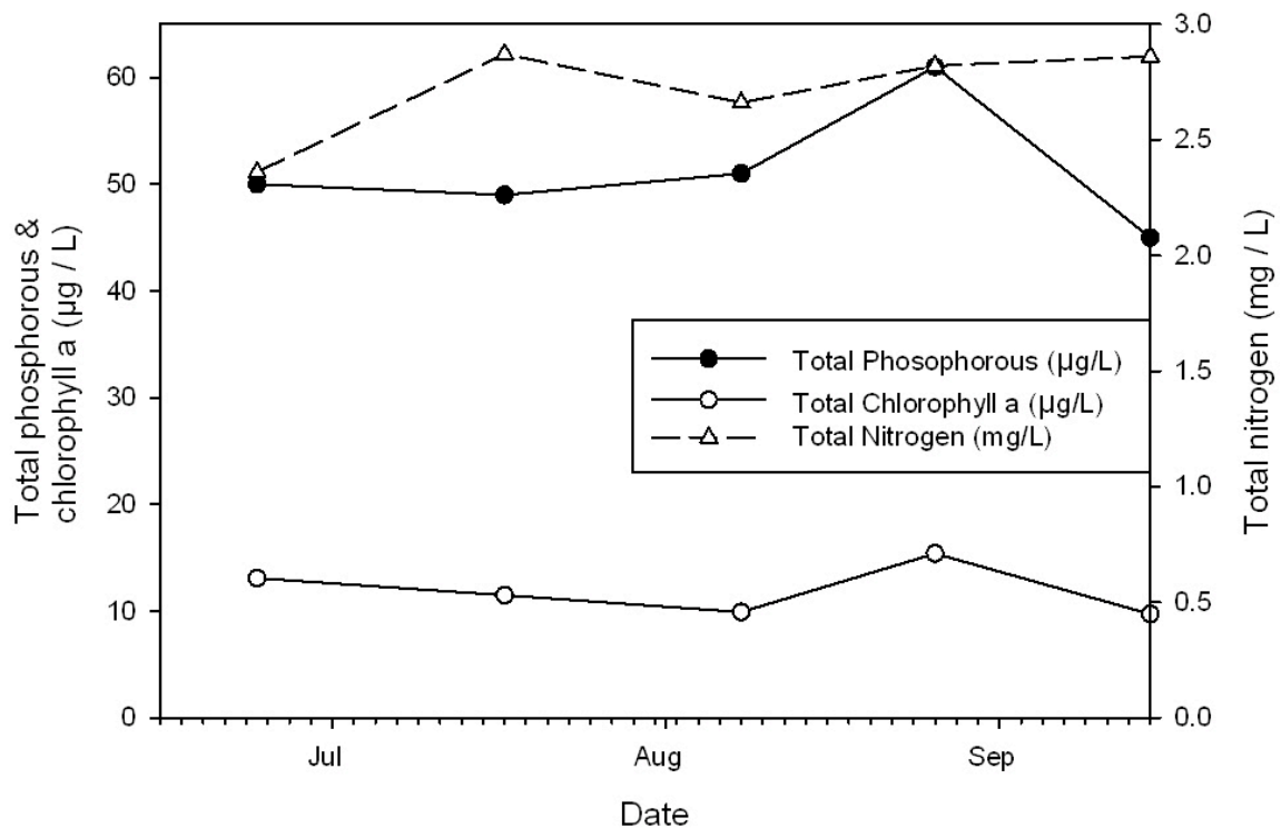
Figure 5. Total phosphorous, chlorophyll a (a measure of algal biomass), and total nitrogen concentrations for Laurier Lake during the summer of 2008.
