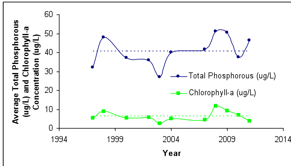
Figure 6 – Historical total phosphorous ( \mu\text{g/L} ) and chlorophyll- a ( \mu\text{g/L} ) concentration averages for Laurier Lake.
