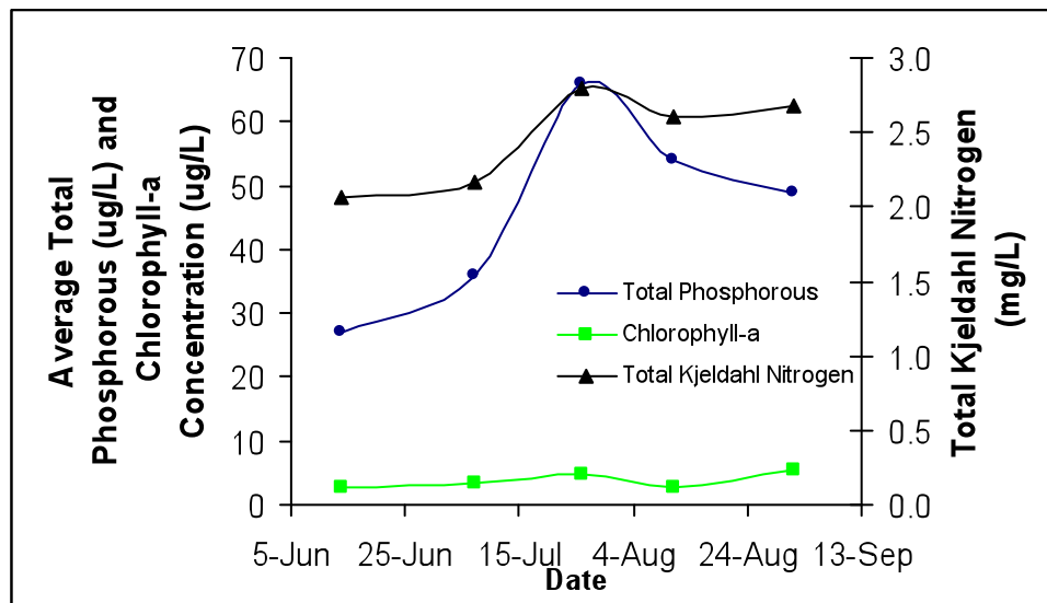
Figure 5 – Total phosphorous (µg/L), chlorophyll-a concentration (µg/L), and total Kjeldahl nitrogen (mg/L), measured five times over the course of the summer at Laurier Lake.
