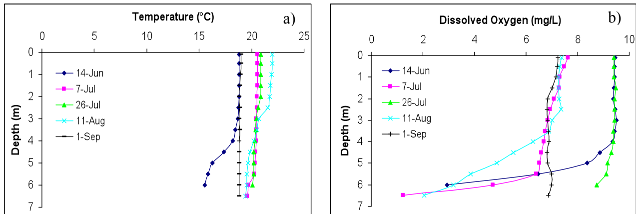
Figure 4 – a) Temperature (°C) and b) dissolved oxygen (mg/L) profiles measured over course of the summer in 2010 at Laurier Lake.
