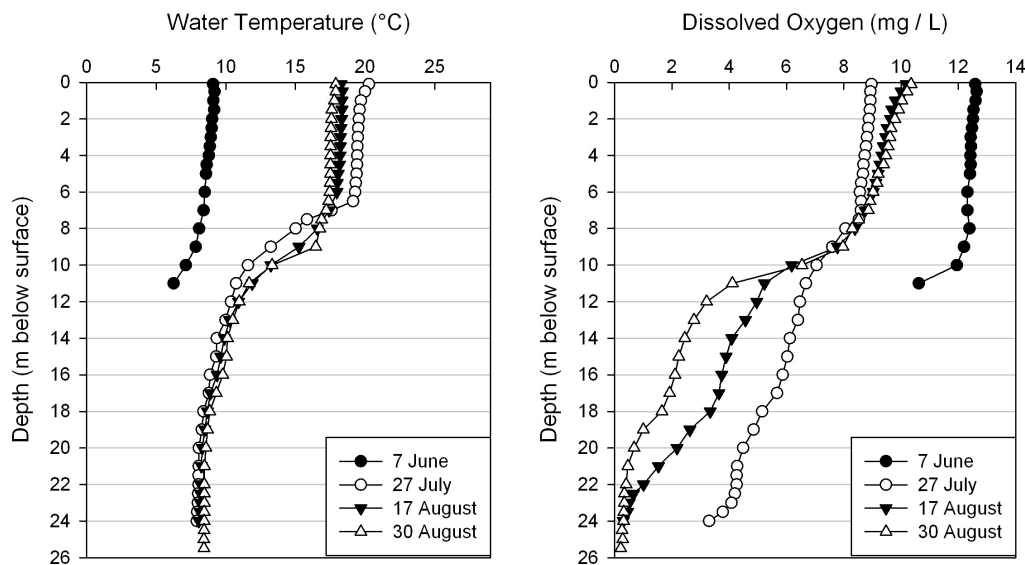
Figure 4. Water temperature ( ^\circ\text{C} ) and dissolved oxygen ( \text{mg/L} ) profiles for Marie Lake during the summer of 2009.
