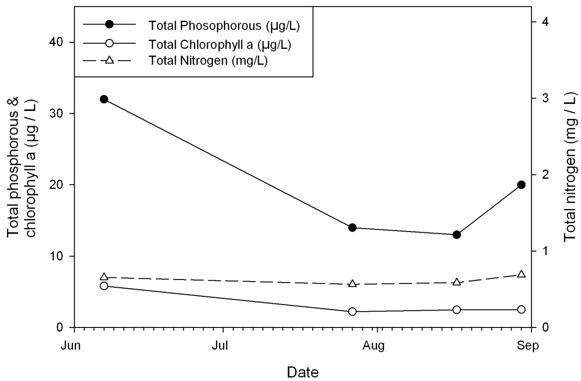
Figure 5. Total phosphorous, chlorophyll a (a measure of algal biomass), and total nitrogen concentrations for Marie Lake during the summer of 2009.
