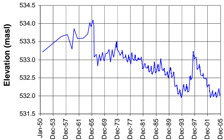
Figure 2. Historic water levels for Moose Lake, 1950 to 2005.
