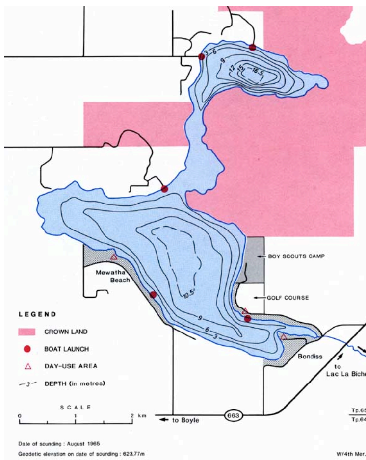
Figure 1: Bathymetry of Skeleton Lake. Each contour represents 3 meters.
