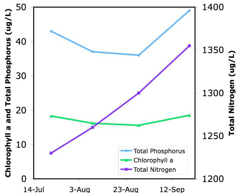
Figure 4: Total phosphorus, total nitrogen & chlorophyll- a (amount of algae) concentrations in Skeleton Lake, summer 2006.
