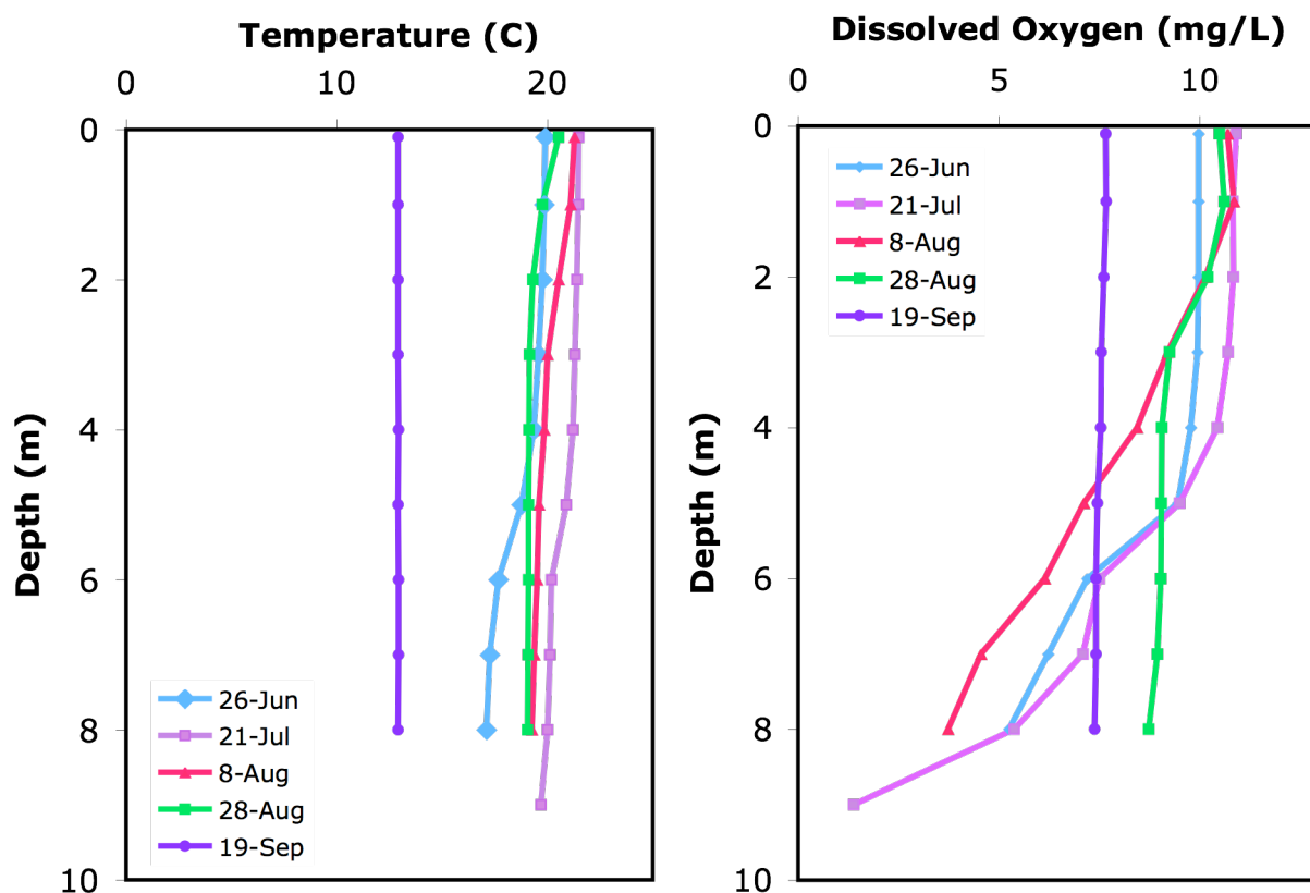
Figures 3 & 4: Temperature and dissolved oxygen profiles in Skeleton Lake, summer 2006.
