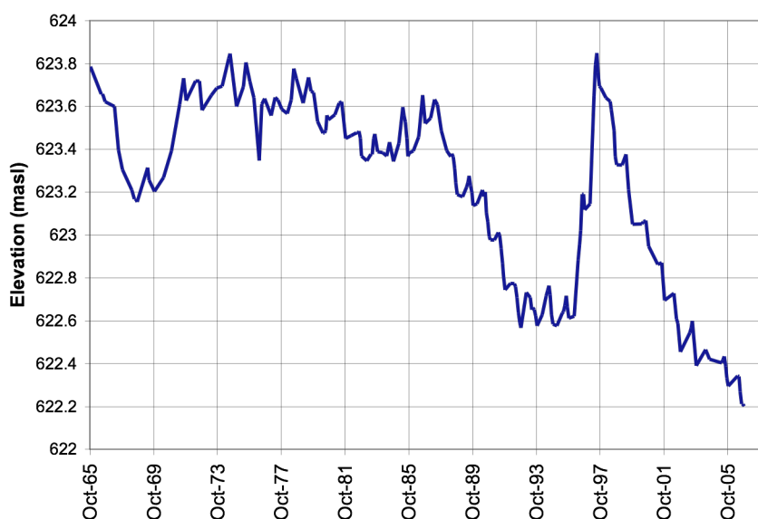
Figure 2: Historical water levels of Skeleton Lake.
