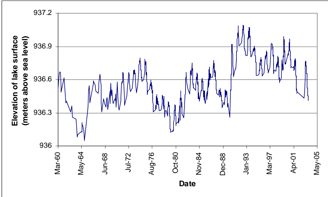
Fig. 2: Water levels in Sylvan Lake for the period of 1960 to 2003.
