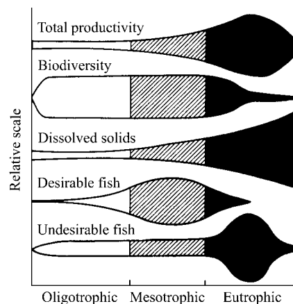
Fig. 9: Suggested changes in various lake characteristics with eutrophication. From “Ecological Effects of Wastewater”, 1980
