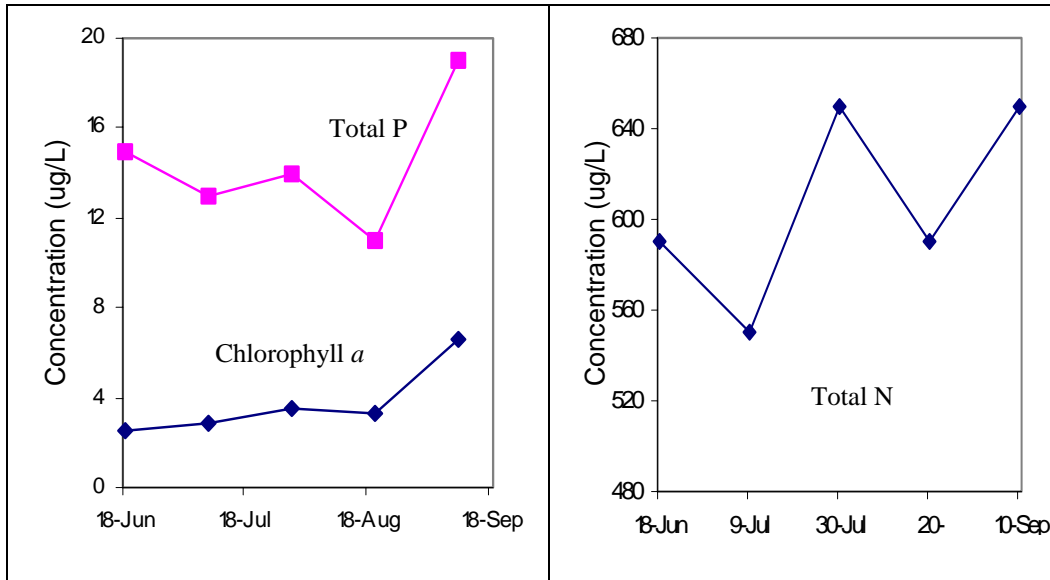
Figs. 5 & 6: Total phosphorus, chlorophyll a and total nitrogen for Sylvan Lake, summer 2003.
