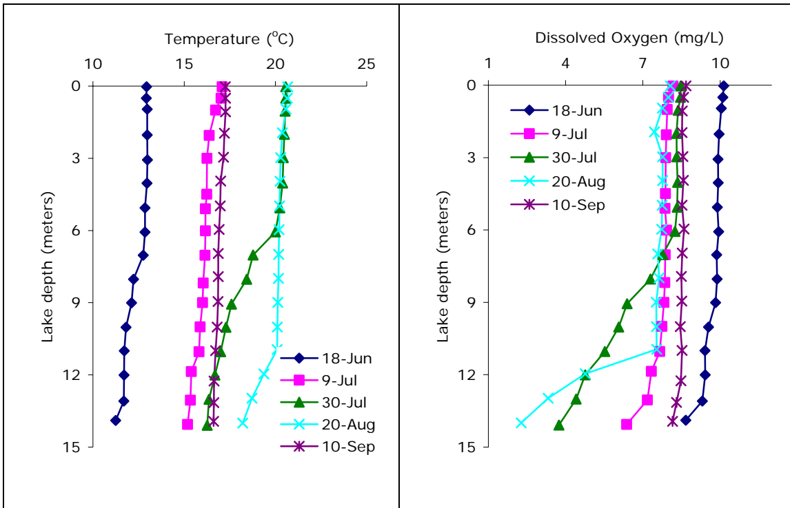
Figs. 3 & 4: Temperature and dissolved oxygen profiles from Sylvan Lake, summer 2003.
