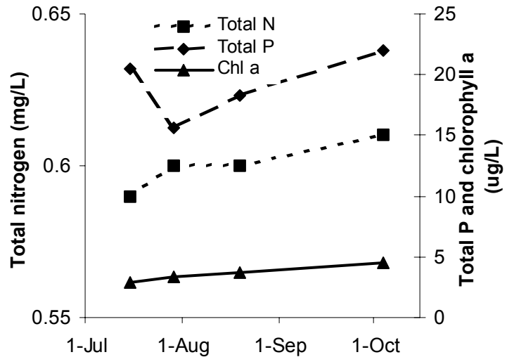
Figure 4. Total phosphorus, total nitrogen and chlorophyll- a (i.e., water greenness concentrations) concentrations in Touchwood Lake, summer 2004.
