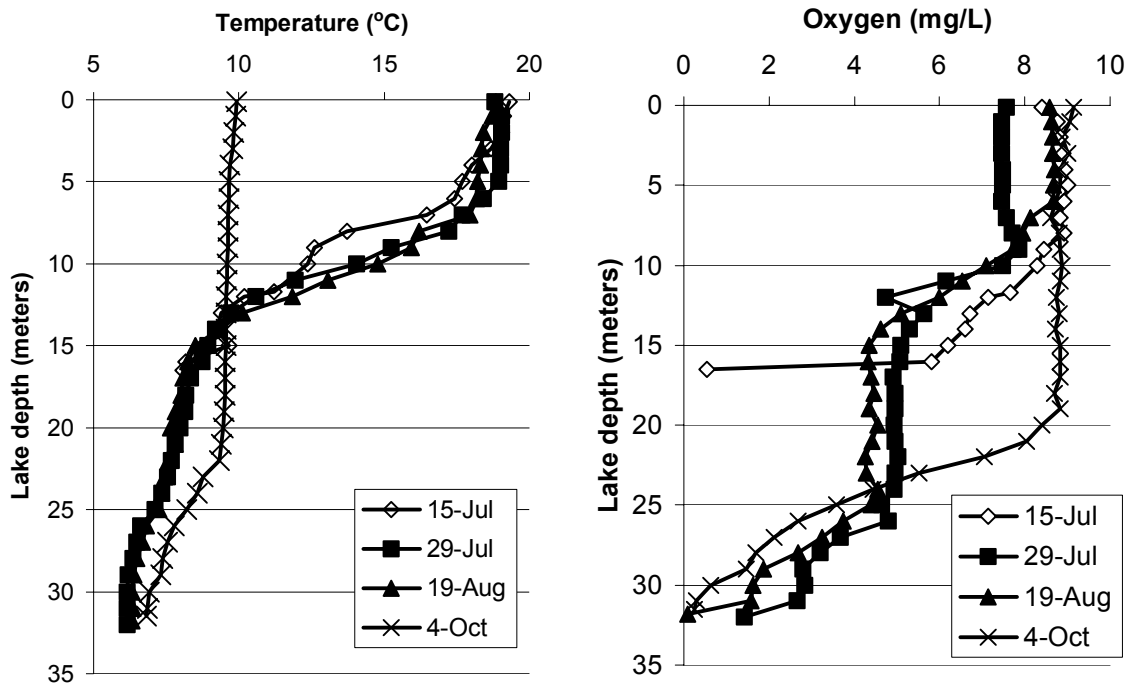
Figure 3: Temperature and dissolved oxygen profiles in Touchwood Lake, summer 2004.
