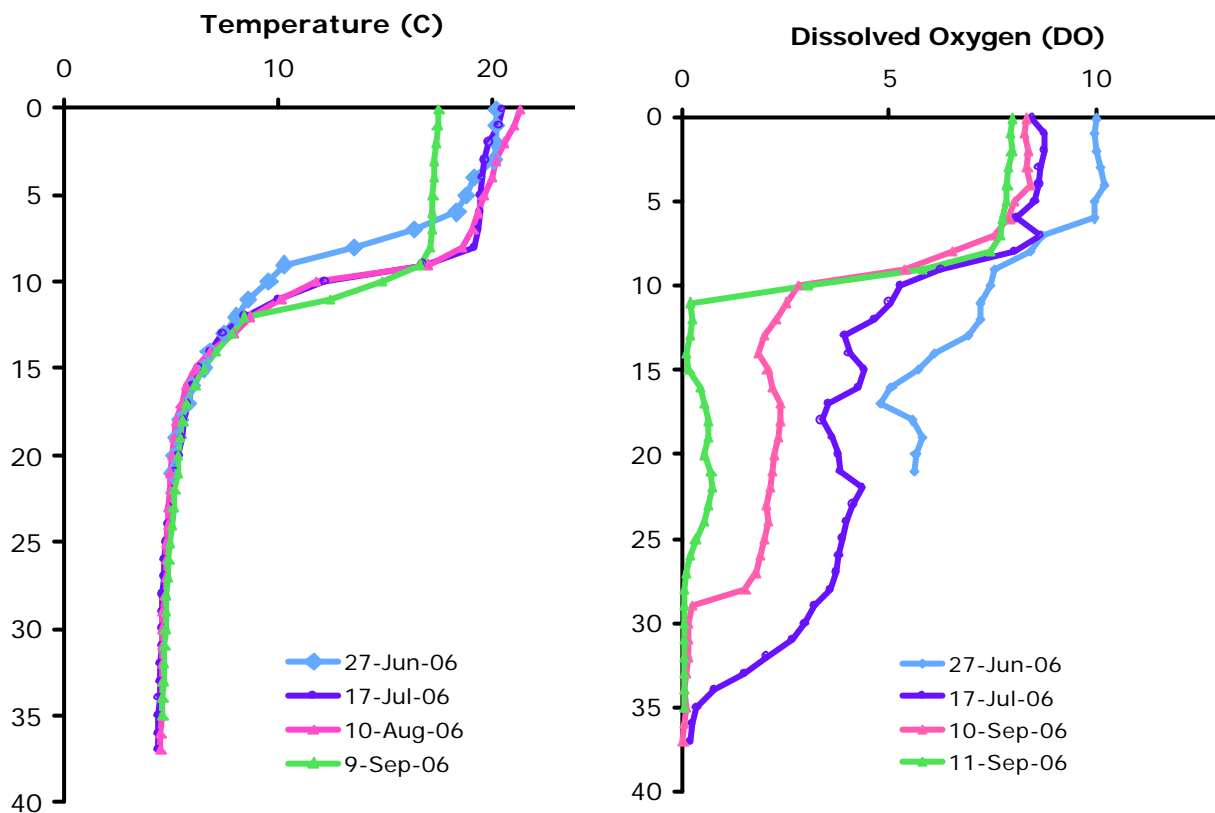
Figure 3. Temperature and oxygen concentration with depth of Wolf Lake, summer 2006.
