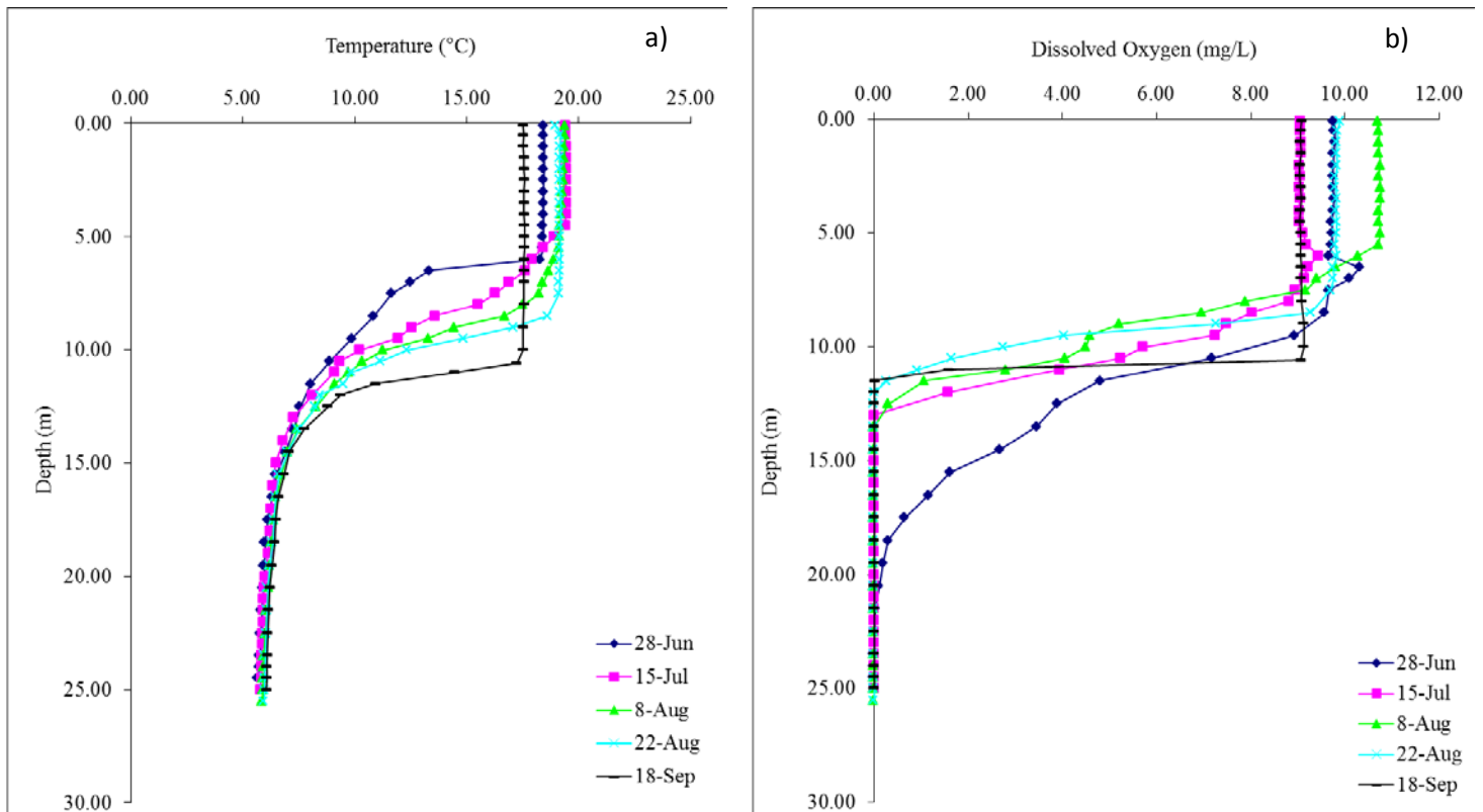
Figure 5 - a) Surface water temperature (°C) and b) dissolved oxygen concentrations (mg/L) measured five times over the course of the summer at Crane Lake.
