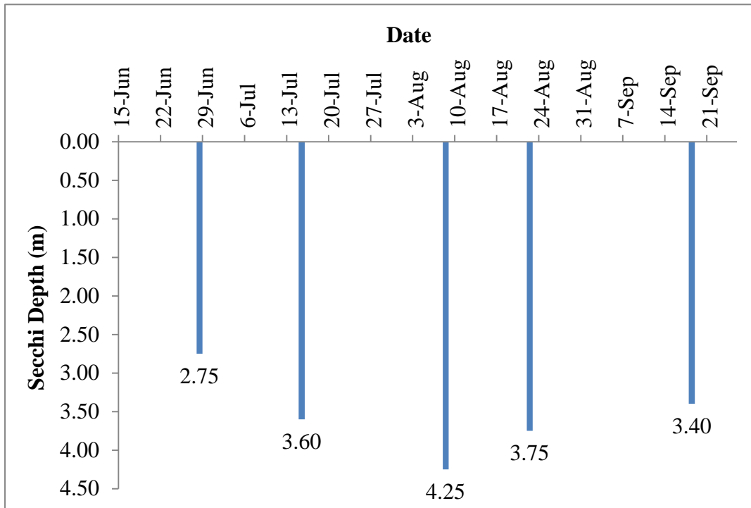
Figure 4 – Secchi disk depth values (m) measured five times at Crane Lake during the summer of 2013.
