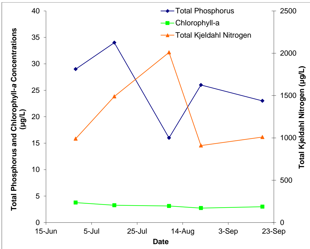
Figure 6 - Total phosphorous ( \mu\text{g/L} ), chlorophyll- a concentration ( \mu\text{g/L} ), and total Kjeldahl nitrogen ( \mu\text{g/L} ) measured five times over the course of the summer at Crane Lake.
