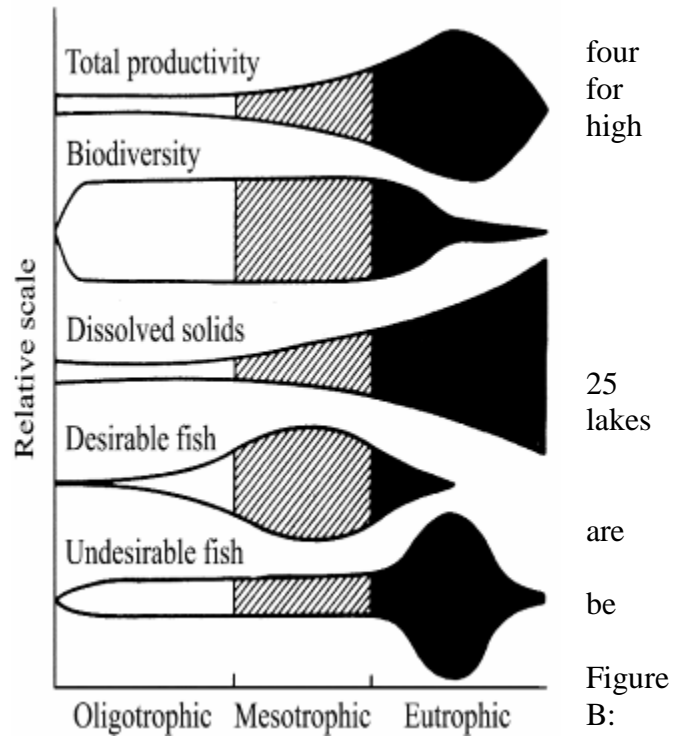
Suggested changes in various lake characteristics with eutrophication. From “Ecological Effects of Wastewater”, 1980.
