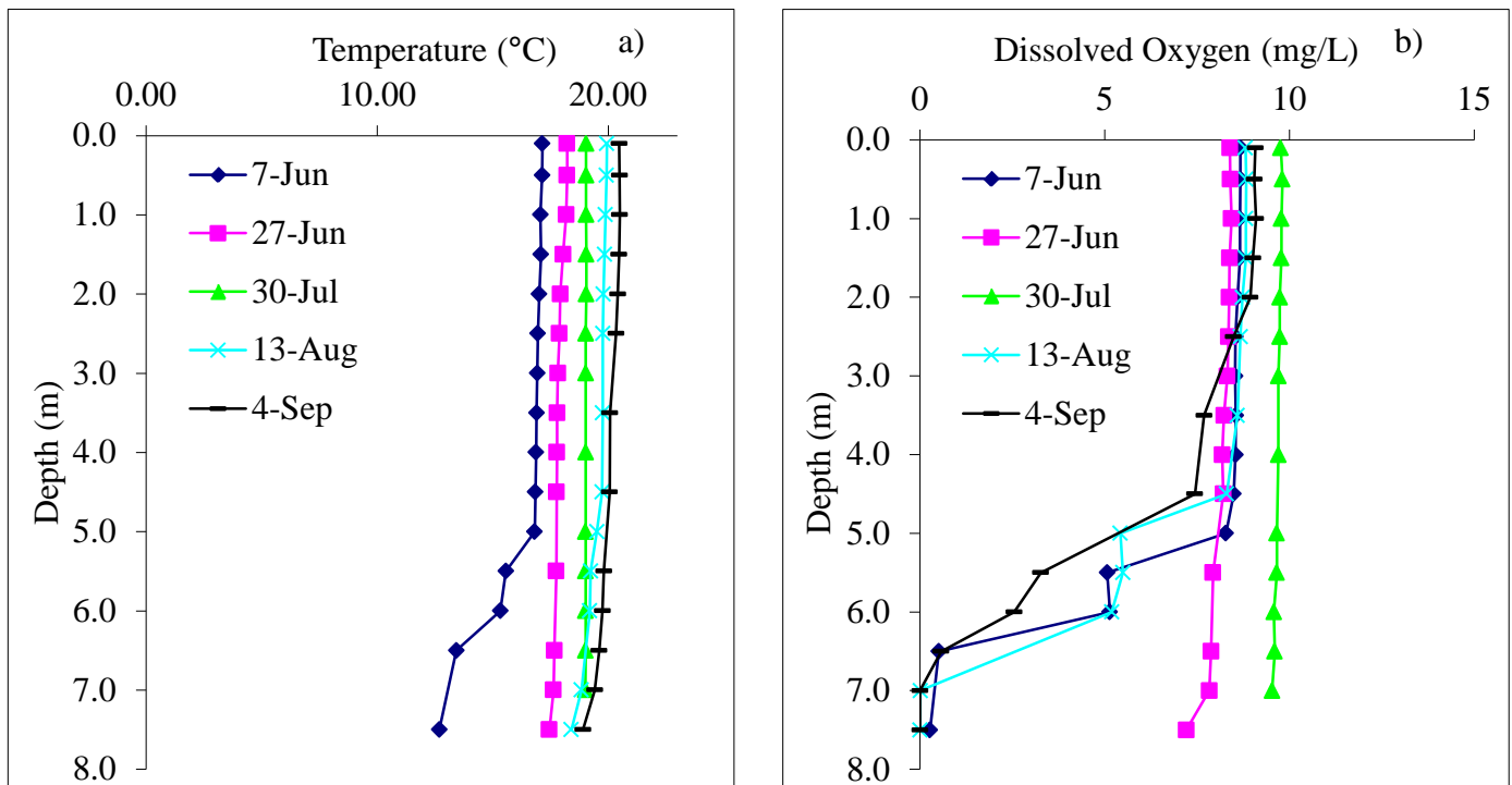
Figure 5 – a) Temperature (°C) and b) dissolved oxygen (mg/L) profiles from Laurier Lake, 2013.
