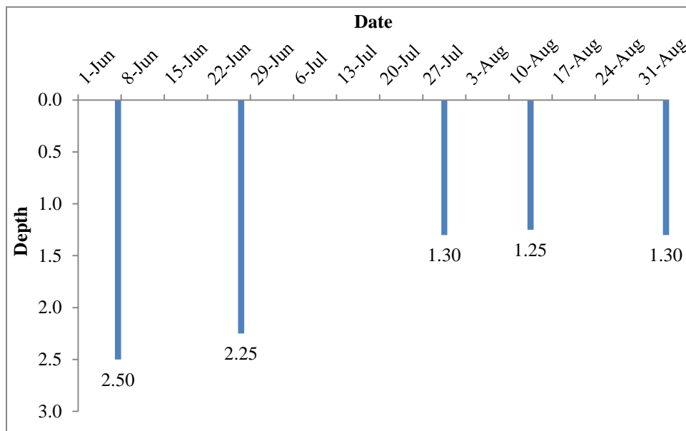
Figure 4 – Secchi disk depths obtained from the profile site on Laurier Lake in 2013.
