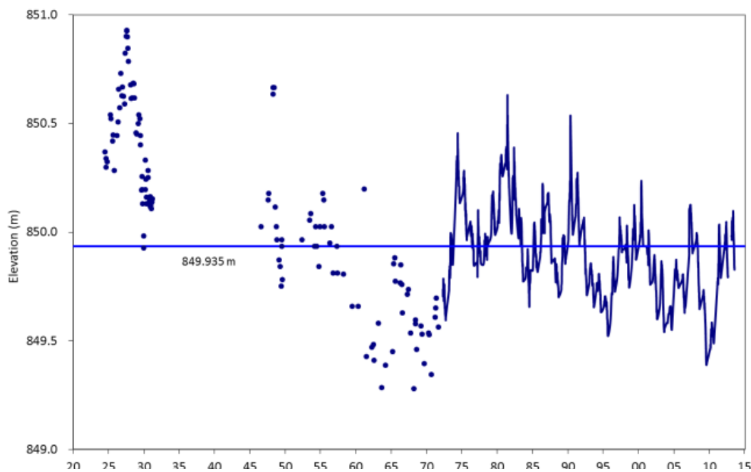
Figure 2 – Historical water levels in meters above sea level measured from 1972-2014.
