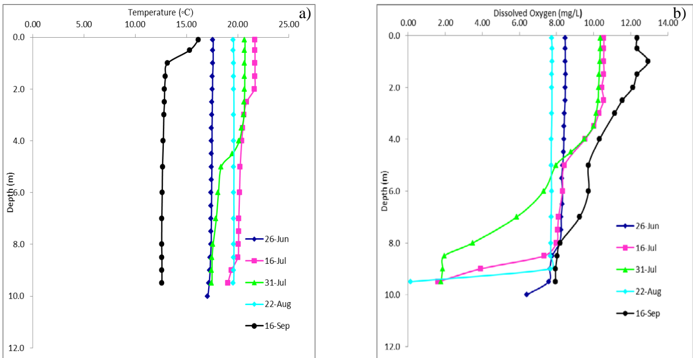
Figure 4 – a) Temperature (°C) and b) dissolved oxygen (mg/L) profiles measured five times over the course of the summer of 2014.
