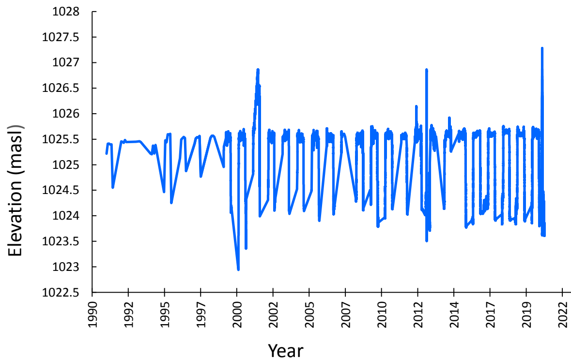
Figure 5. Water levels measured in meters above sea level (masl) from 1991-2020. Data retrieved from Environment Canada (1991 – 1998), and Alberta Environment and Parks (1999-2020).
