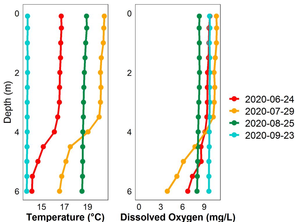
Figure 4. a) Temperature (°C) and b) dissolved oxygen (mg/L) profiles for Chestermere Lake measured four times over the course of the summer of 2020.
